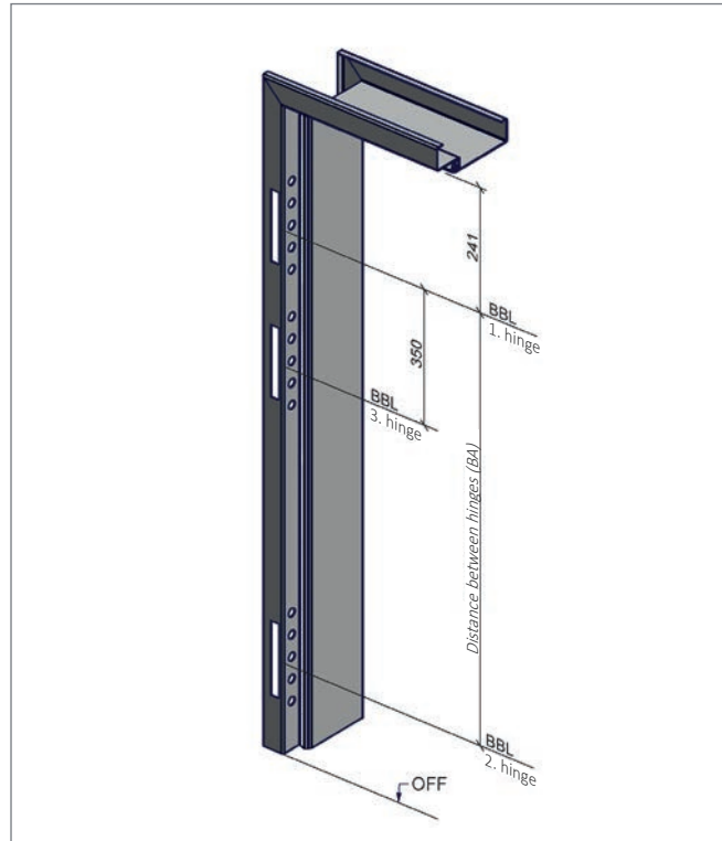
Hinge positions · Hinge pockets BVX11000 · Illustration: 3 hinge pockets
