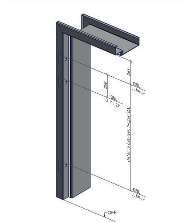
Hinge positions · Hinge pockets V8618 and BTV10200 · Illustration: 3 hinge pockets
