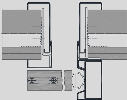
Illustration for stud and brick walls.
