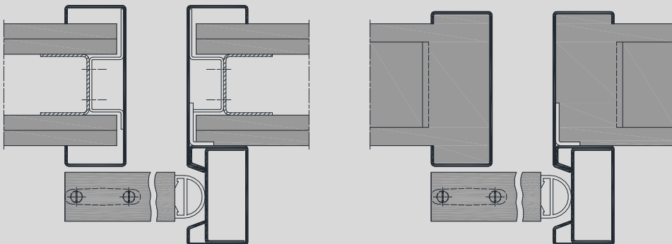
Illustration for stud and brick walls.
