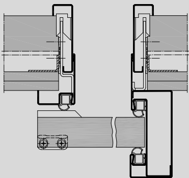
Illustration for stud and brick walls.
