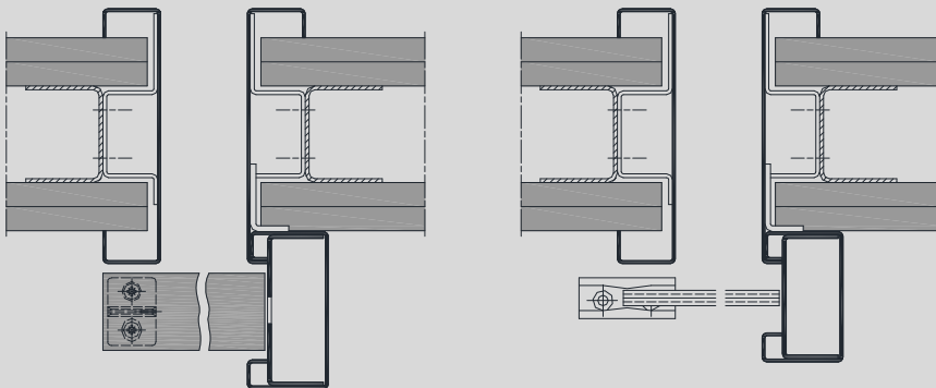
Timber door leaf
