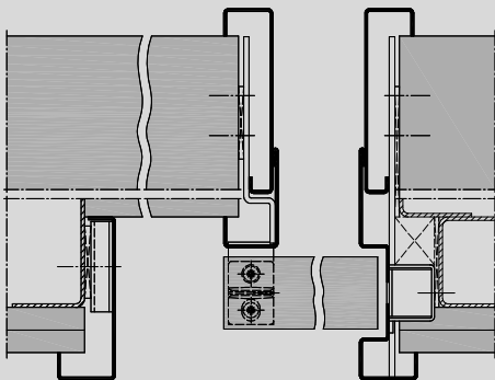
Version with timber door leaf, illustration for stud and brick walls.
