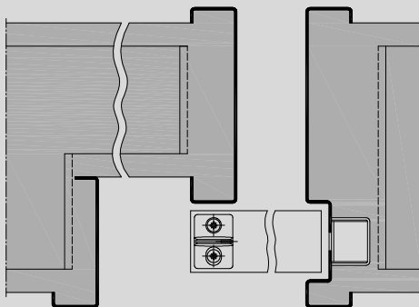
Version with timber door leaf, illustration for brick walls.
