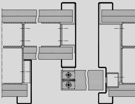
Version with timber door leaf, illustration for stud walls.
