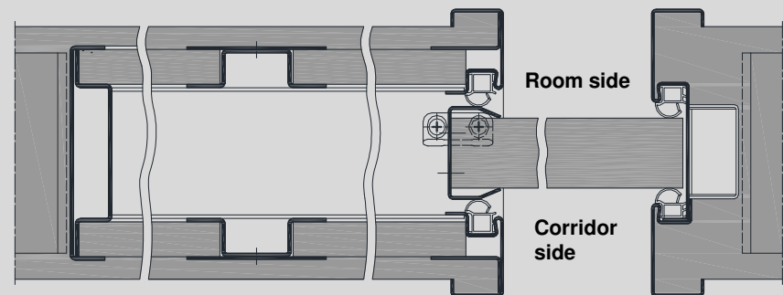
Room side with inspection cover strip
