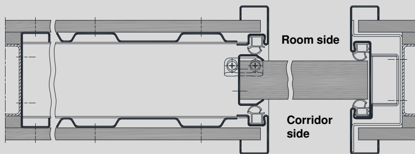
Corridor side without inspection cover strip
