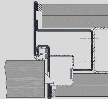
Top-light with tube glazing beads
