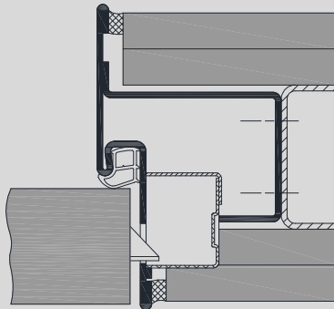
Concealed hinge
