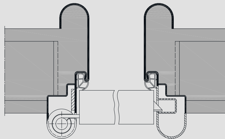
Vision panel with inner blind
