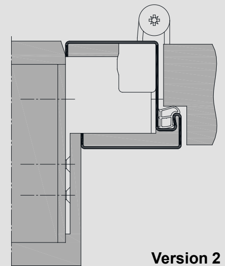
VX-hinge, version 2 top-light with tube glazing beads
