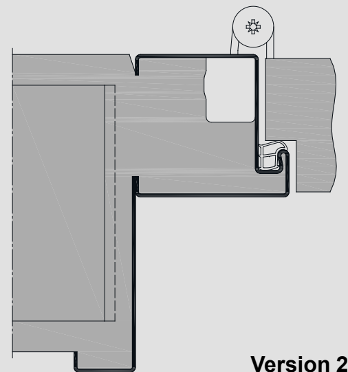
VX hinge, version 2 top-light with tube glazing beads
