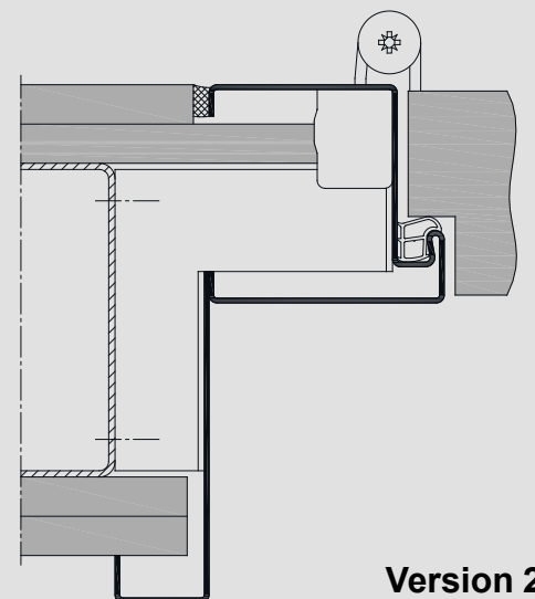
VX hinge, version 2 top-light with tube glazing beads
