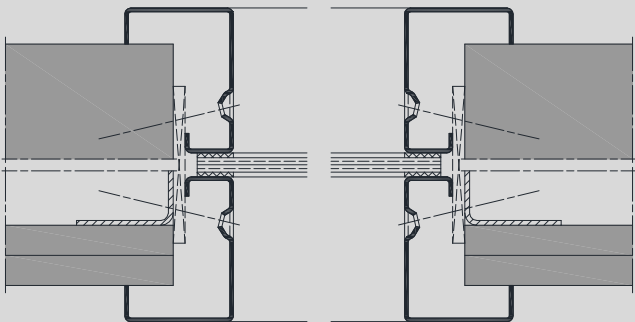
Illustration for stud and brick walls.
