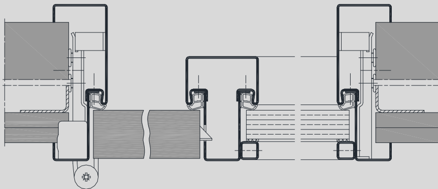
Version with flush closing door leaf, illustration for stud and brick walls.
