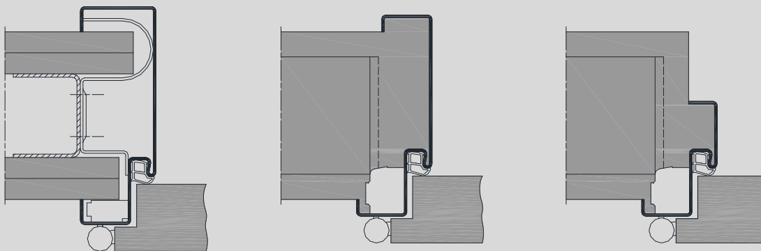
Version with rebated door leaf, illustration for stud and brick walls.
