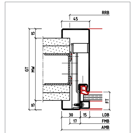
15ZBud (VG-Nd)-Fensterzarge
