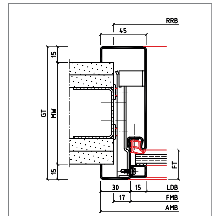
15ZBud (VG-Nd)-Fensterzarge
