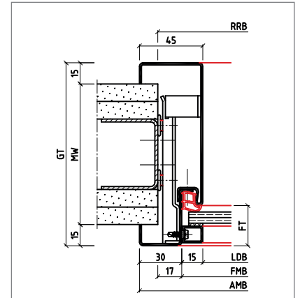
15ZBud (VG-Nd)-Fensterzarge
