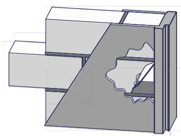
- Fester Steinanker
